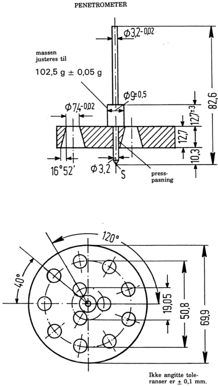
Figur 1 - Penetrometer
